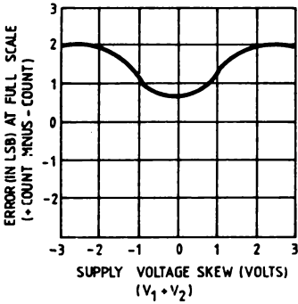
Rollover Error vs Power Supply Skew
