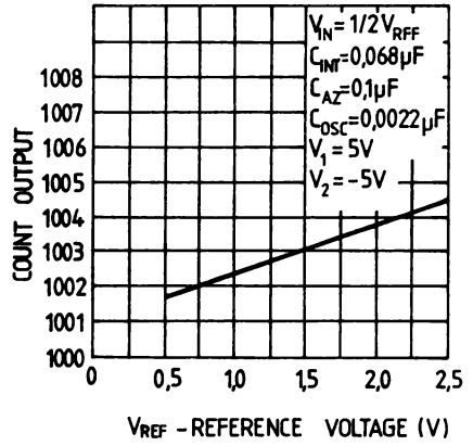
Ratio Operation ( V_{IN}/V_{REF} = \text{Constant} )
