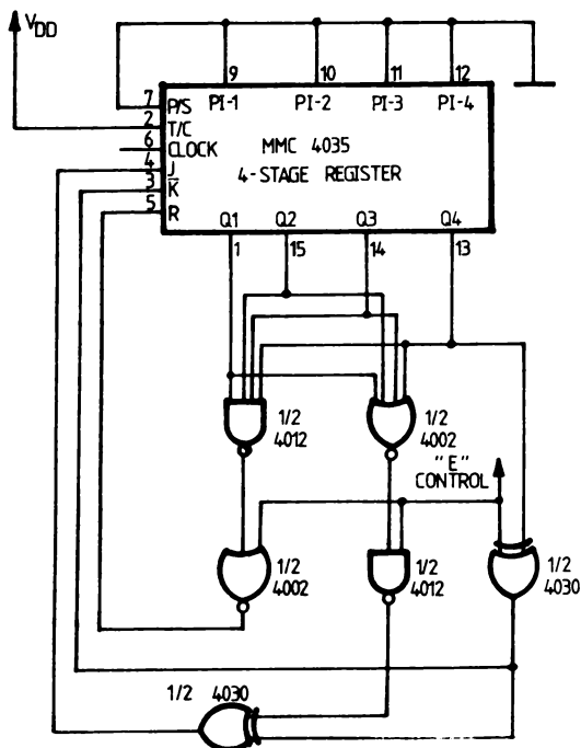
Double sequence generator
