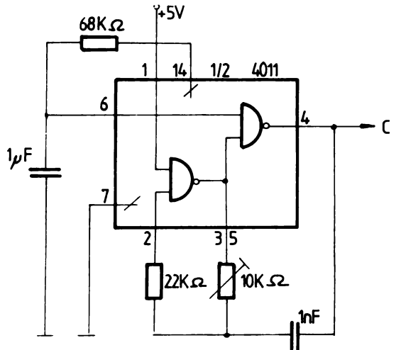
FIG.6 THE DELAYED CLOCK CIRCUIT
