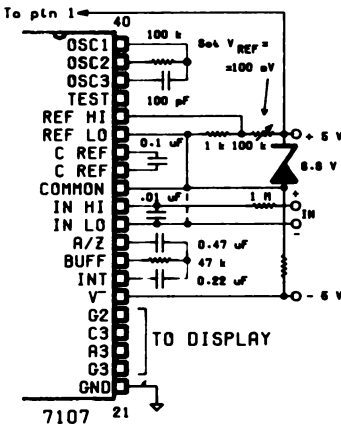
Fig.3 7107 with Zener diode reference. Since low T. C. Zeners have breakdown voltage \approx 6.8 V , diode must be placed across the total supply (10V). IN LO may be tied to either COMMON or GND
