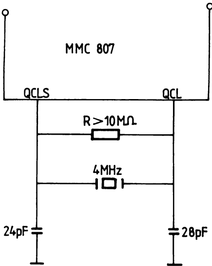
EXTERNAL NETWORK OF EMITTER'S OSCILLATOR
