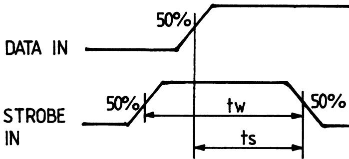
Data setup time and strobe pulse duration
