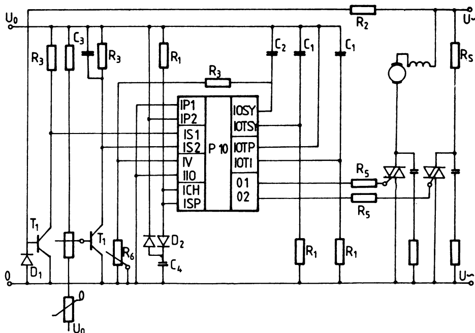
Fig.8 System with phase control (O1) and burst control (O2) for two independent loads
