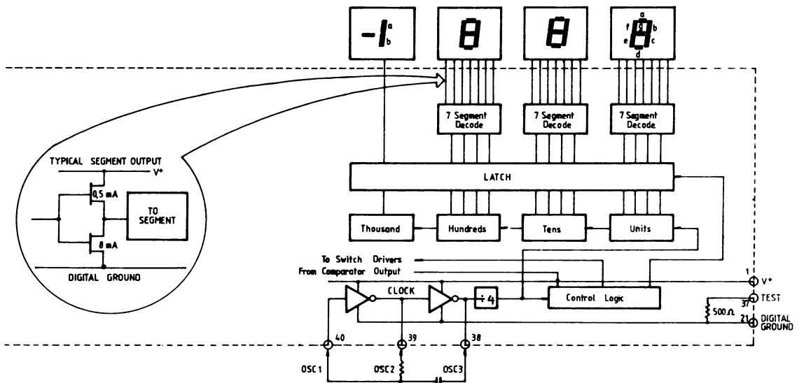
Figure 8: Digital Section 7107
