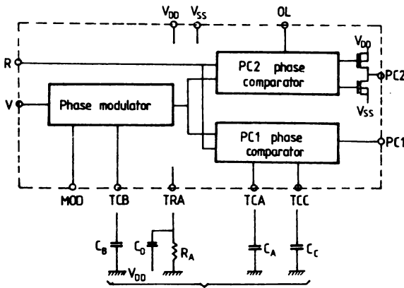
external circuitry
