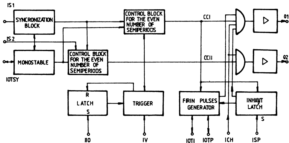
Fig.3c Block diagram in P011 program
