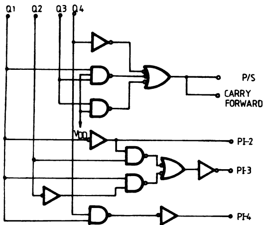
BIDEDEC logic
