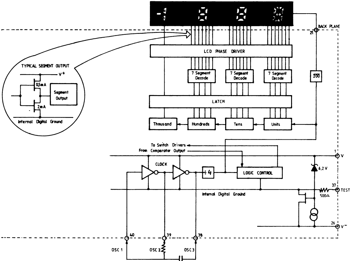
Figure 7: Digital Section 7106
