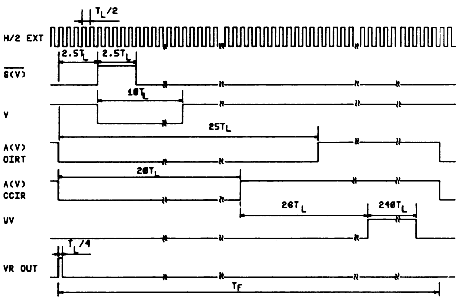
Fig. 6 Vertical timing T_F = 262.5T_L for 525/625-V DD ; T_F = 312.5T_L for 525/625-V SS . only for 525/625-V SS .
