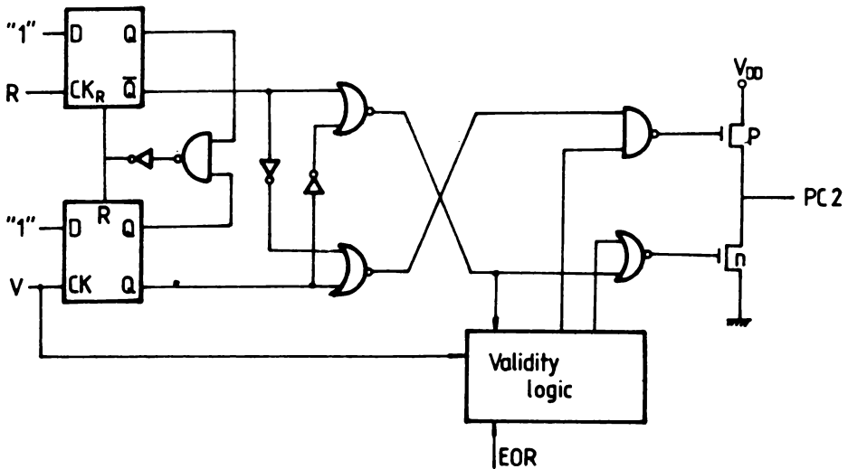
Simplified logic diagram of the PC2 comparator
