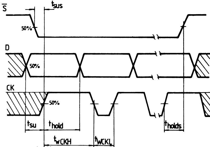
MMC 356 — Loading waveforms
