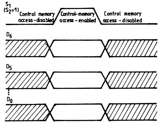
MMC 356 — Loading waveforms
