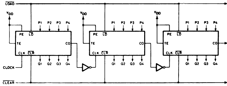
Cascaded counter packages in the ripple-clocked mode.
