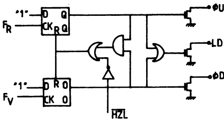
Phase and frequency comparator
