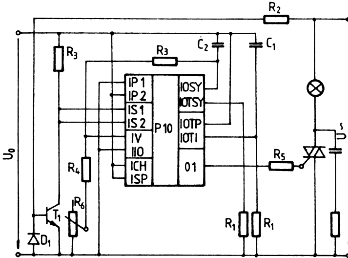
Fig.4 Simple AC regulator
