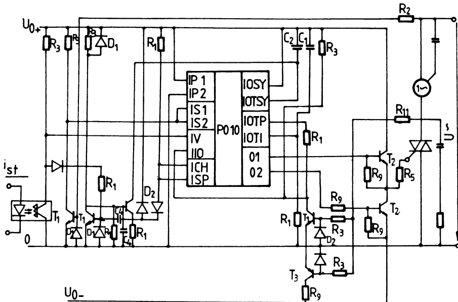
Fig.7 AC Switch
