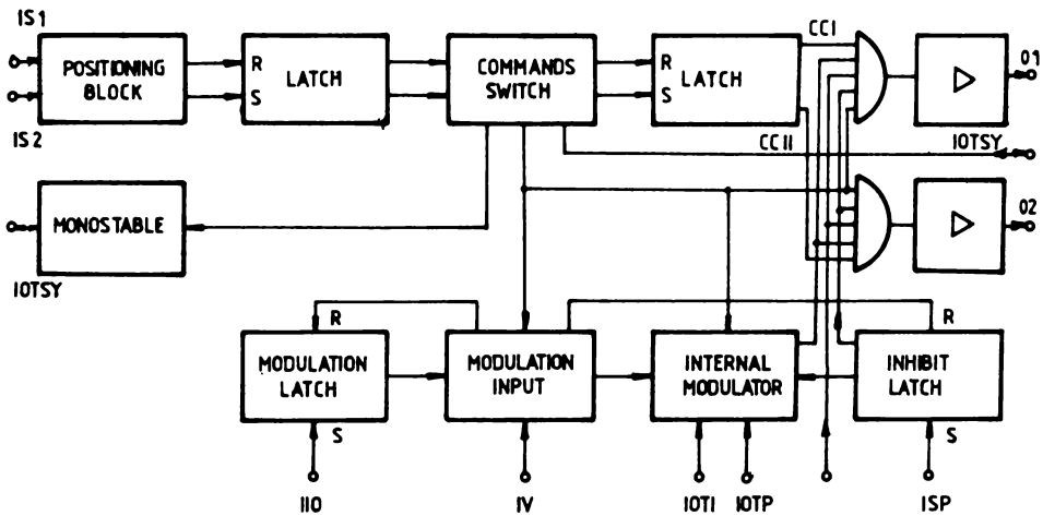
Fig. 3e. BLOCK DIAGRAM IN P11 PROGRAM
