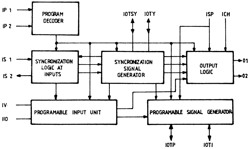
Fig. 2 Block diagram
