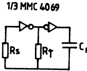
Typical RC oscillator circuit
