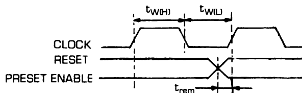
Timing diagram defining t_{rem}
