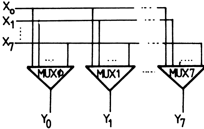
Crosspoint array
