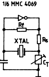
Typical crystal oscillator circuit
